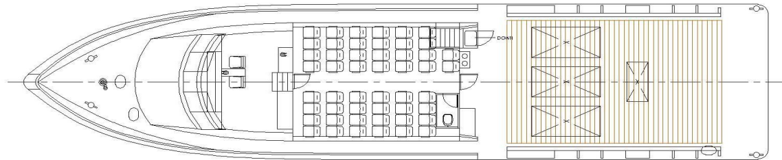
PLAN - MAIN DECK
