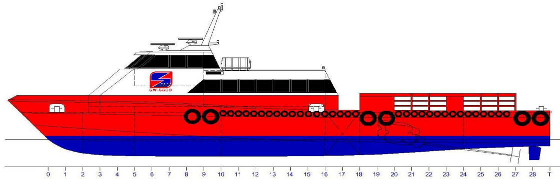
OUTBOARD PROFILE
